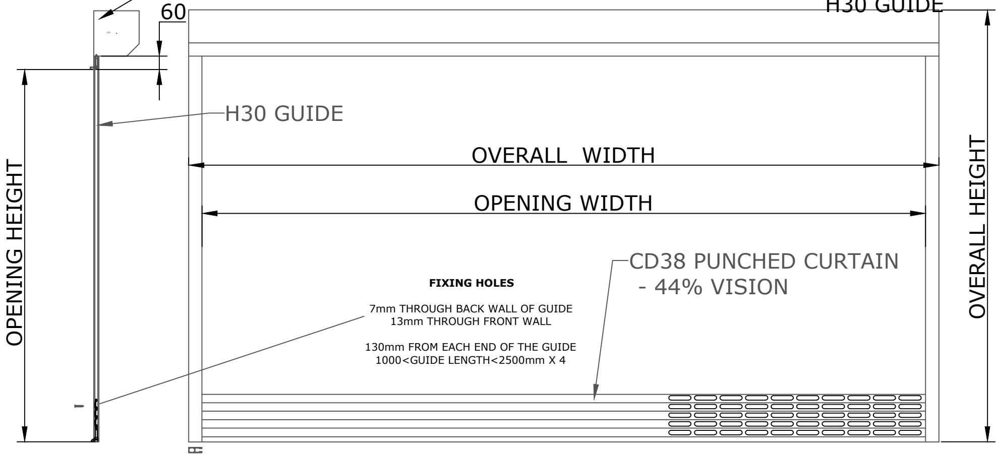
CD38 SINGLE SKIN SLAT
