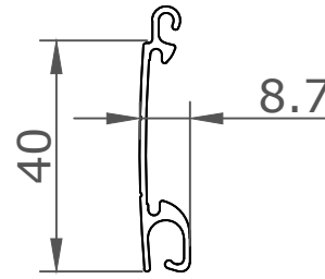
CD38 SINGLE SKIN SLAT
